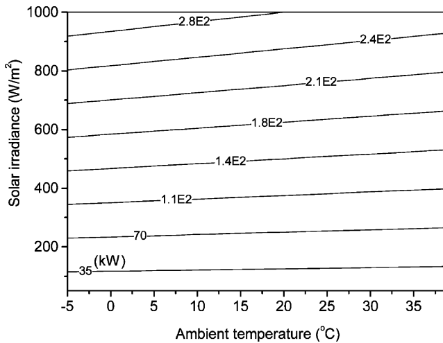
Fig. 2. Effect of ambient temperature and solar irradiance on power generation.
