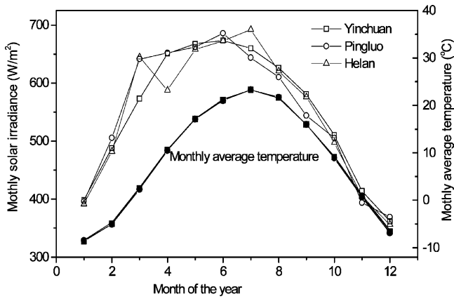
Fig. 4. Monthly average temperature and solar irradiance at three different regions.
