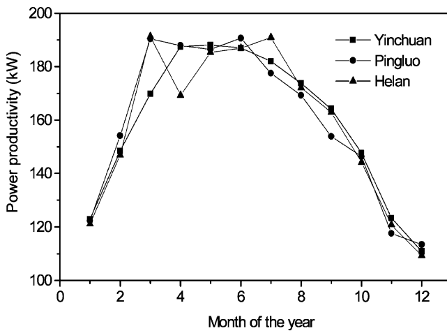
Fig. 5. Monthly average solar power plant generation rate at three different regions.
