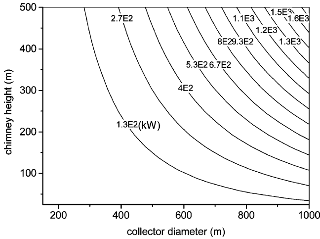
Fig. 3. Effect of solar chimney height and diameter of collector on power generation.
