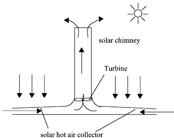
Fig. 1. Schematic diagram of a solar chimney power plant.
